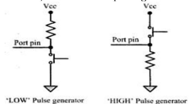
Fig. 3.7: Push Button Switch Configuration
