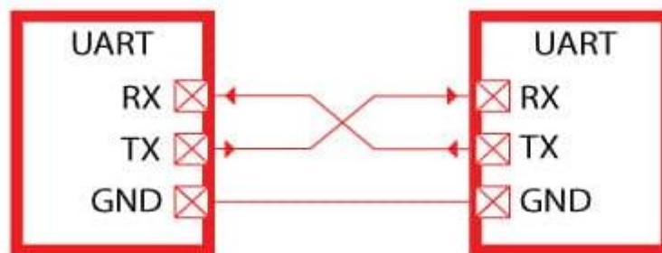
Fig. 3.9: UART Interfacing
